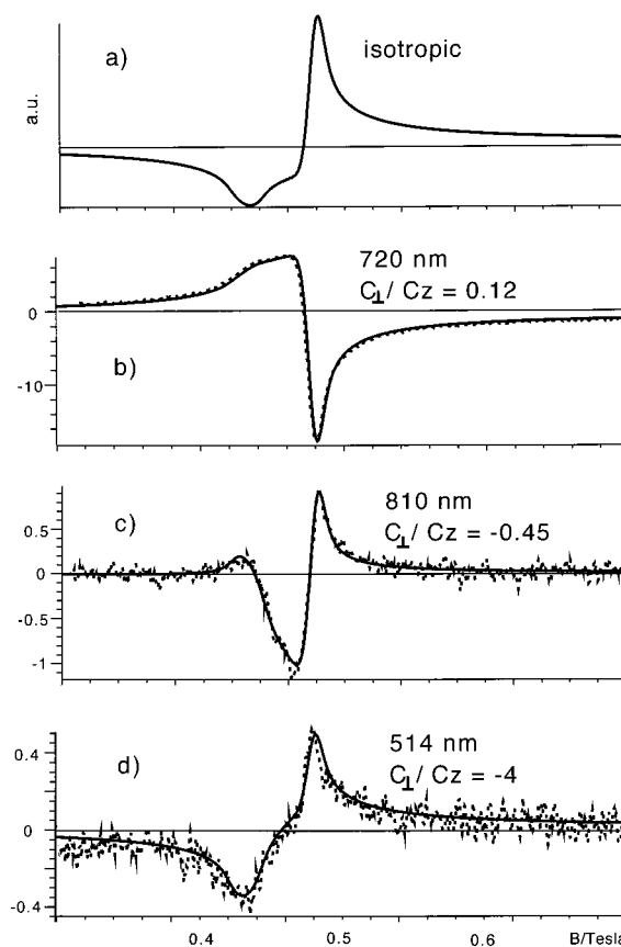
Figure 2. Dispersion type ODEPR spectra of azurin at different optical wavelengths in units of \Delta\epsilon_x \times 10^{-3} \text{ M}^{-1} \text{ cm}^{-1} (dashed line). Fit curves were calculated according to eq 2 (solid line).
